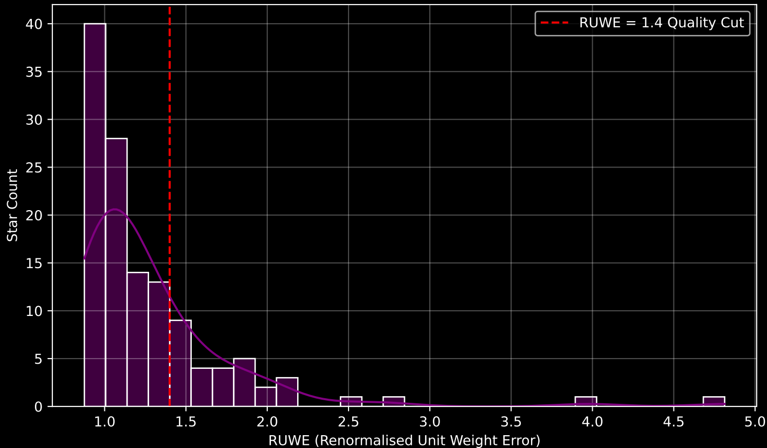
GAPOGEE DR17 Field [121+74_MGA] RUWE Distribution (n= 126)
