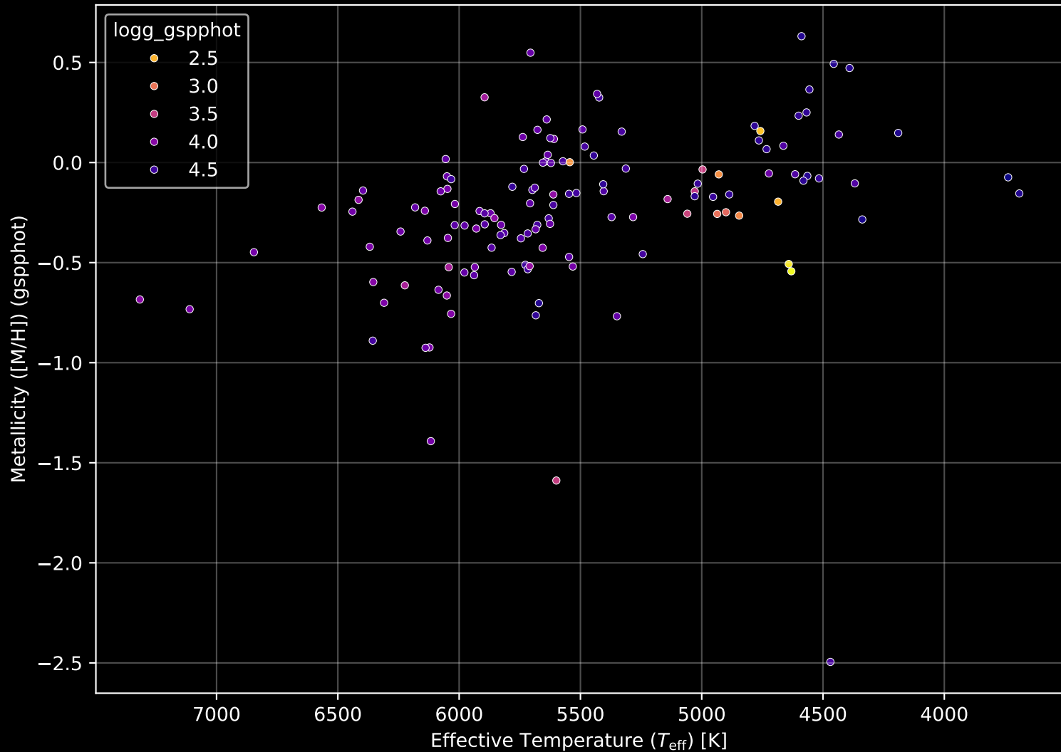
APOGEE DR17 Field: [121+74_MGA] Stellar Population Parameters (n= 134)
