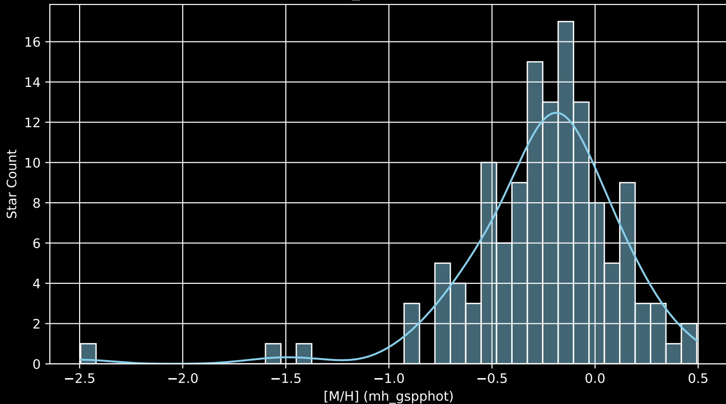
APOGEE DR17 Field: [121+74_MGA [M/H] (mh_gspphot) (n= 132)
