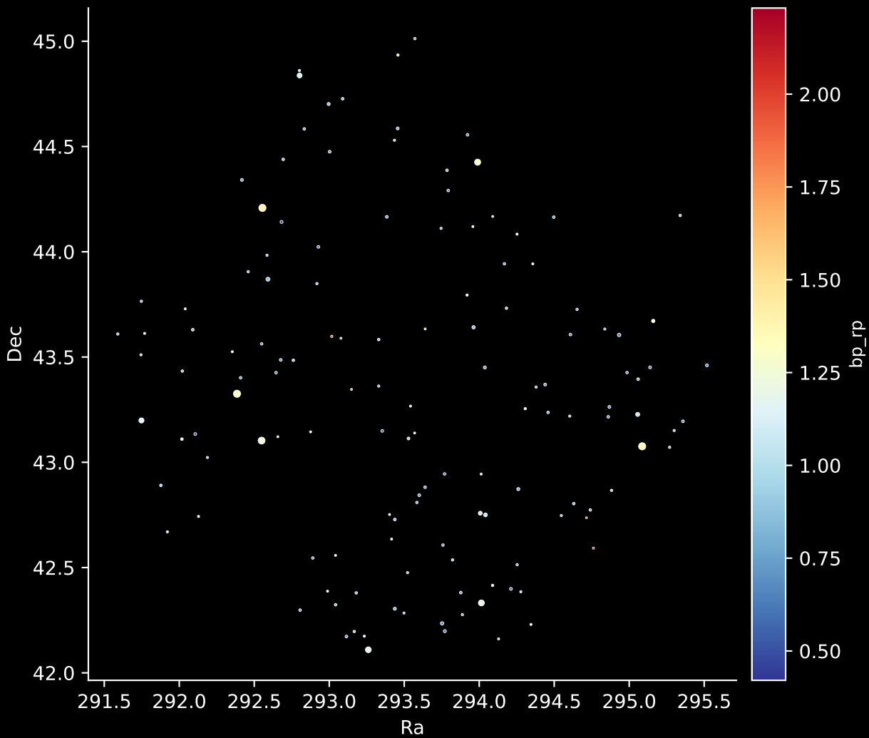
APOGEE DR17 Field: [121+74_MGA] Stars: 134
