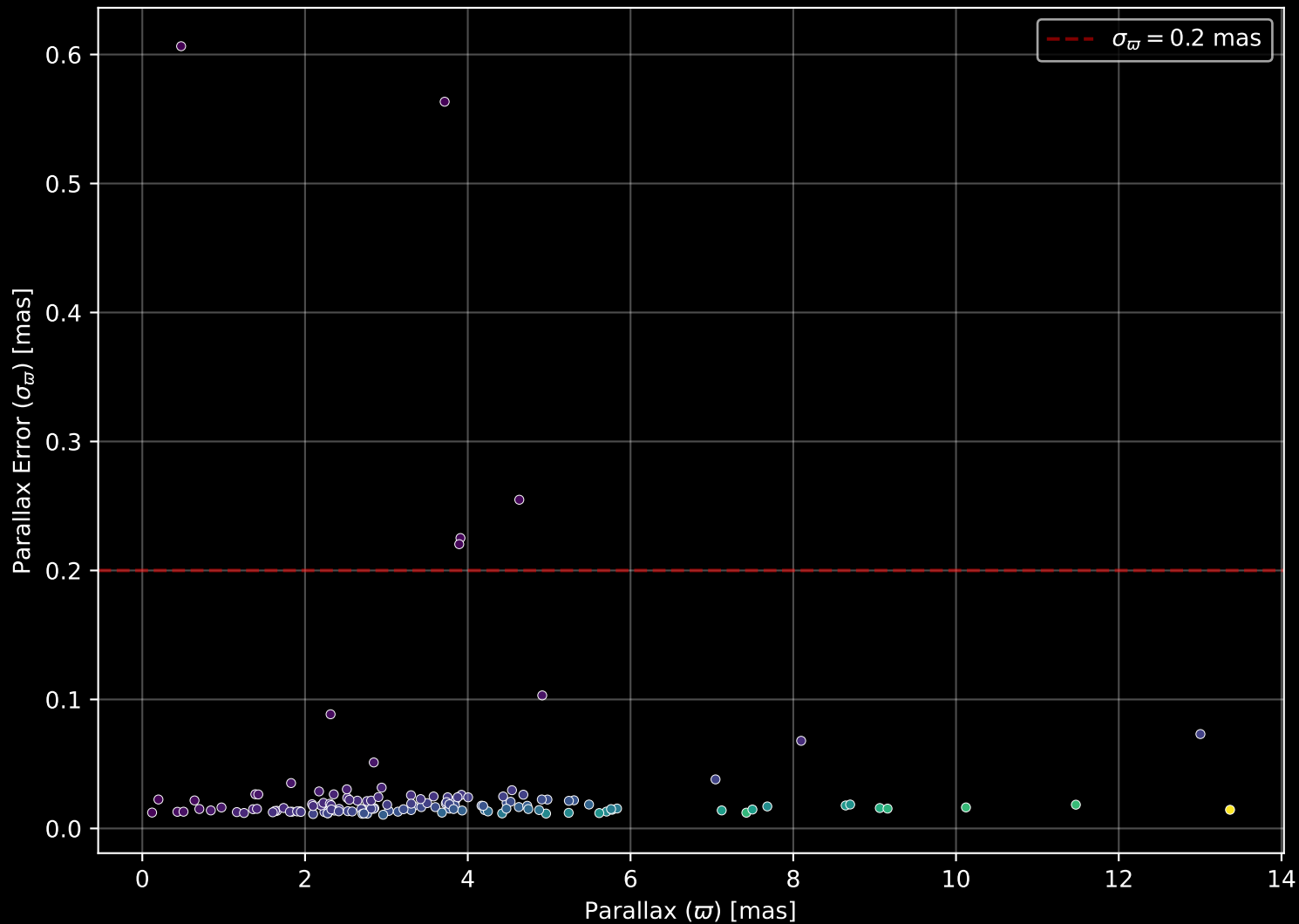
APOGEE DR17 Field: [121+74_MGA] Parallax Quality (n= 134)
