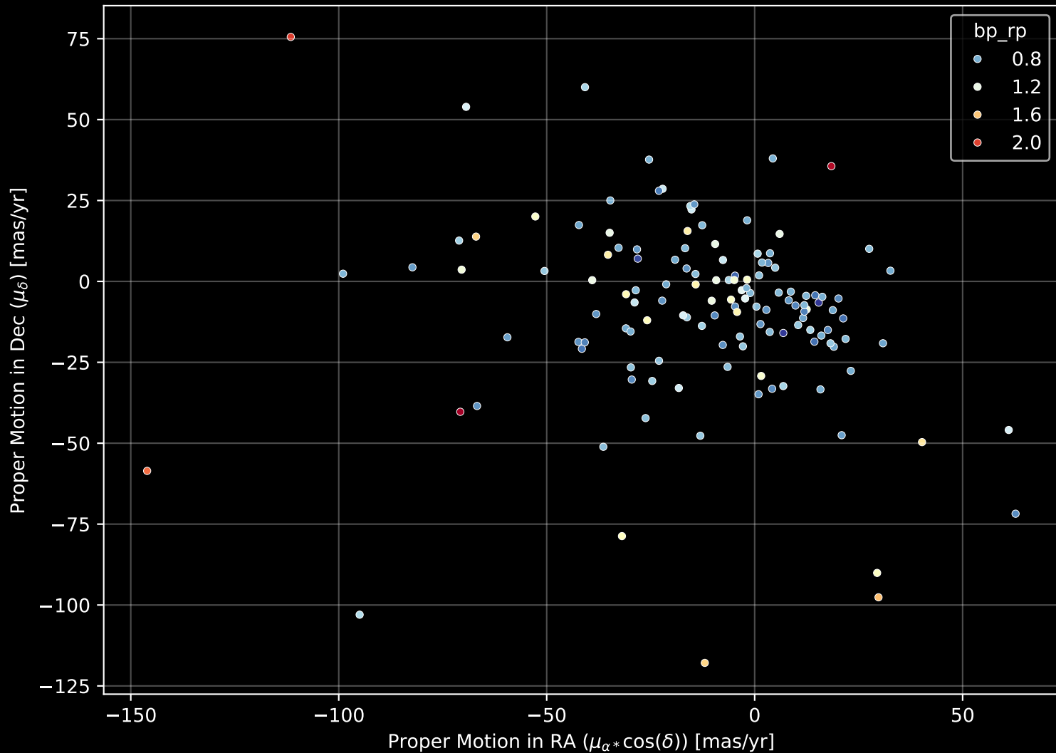
APOGEE DR17 Field: [121+74_MGA] Proper Motion Diagram (n= 134)
