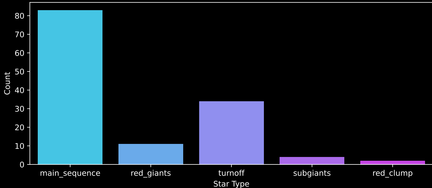
APOGEE DR17 Field: [121+74_MGA] Count plot of Star Type
